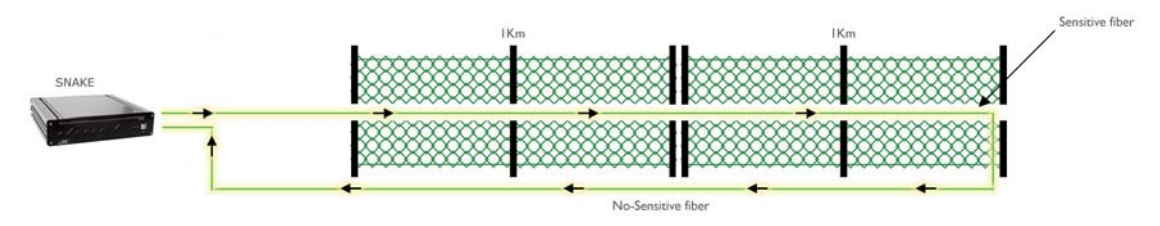
SNAKE™ provides indications of fault, pre-alarm, alarm and fibre cut via an RS485 serial line, for all the monitored channels.
